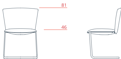
Visitors low-backrest chair, cantilever base 1VE2010 L 57 P 55 H 81
