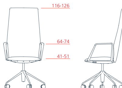
Executive high-backrest armchair with aluminium armrest, 5-star swivel base on castors, adjustable height 1VE5534 L 63 P 71 H 116-126
