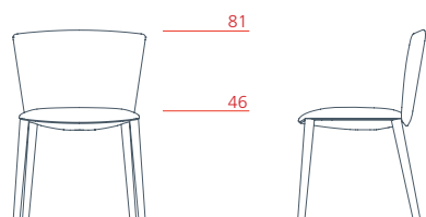
Visitors low-backrest chair, 4 wooden leg base 1VE1010 L 57 P 55 H 81
