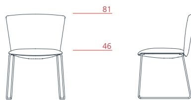
Visitors low-backrest chair, sled base 1VE3010 L 60 P 55 H 81
