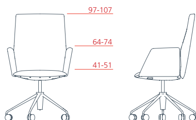
Executive medium-backrest armchair with upholstered armrest, 5-star swivel base on castors, adjustable height 1VE5522 L 63 P 69 H 97-107
