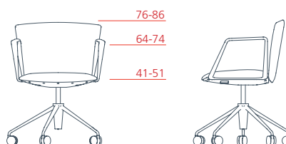
Executive low-backrest armchair with aluminium armrest, 5-star swivel base on castors, adjustable height 1VE5514 L 63 P 69 H 76-86
