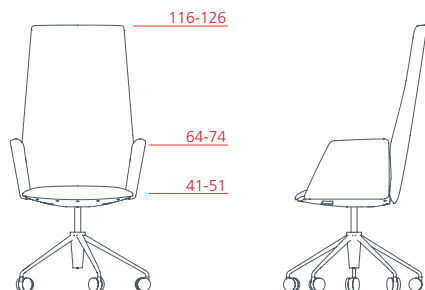
Executive high-backrest armchair with upholstered armrest, 5-star swivel base on castors, adjustable height 1VE5532 L 63 P 71 H 116-126
